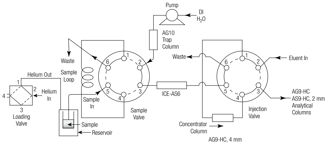
Figure 2. Loading the sample loop.
