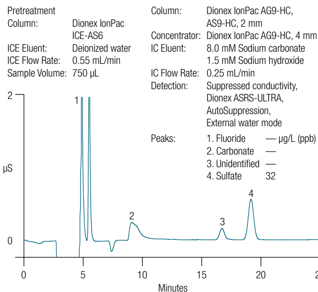
Figure 9. Representative system blank.
