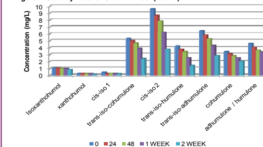
Figure 4. Stability Data for Ultra IPA Beer (Beer 1).
