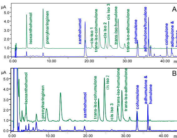
FIGURE 3. Chromatograms of A. Bitter Acids Standard Mixture; B. Ultra IPA Beer Sample. Blue Trace at 550 mV, Green Trace at 850 mV.
