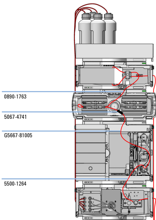
Figure 1 Capillary Connections
